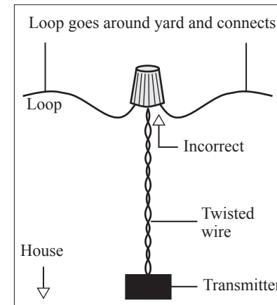
Incorrect Neutral Zone Wire Splicing
