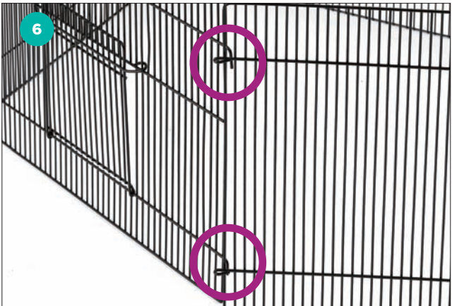
STEP 6 Slide the pin in the center of the panel through its corresponding loop on the adjacent panel. Repeat with the pin at the bottom .
