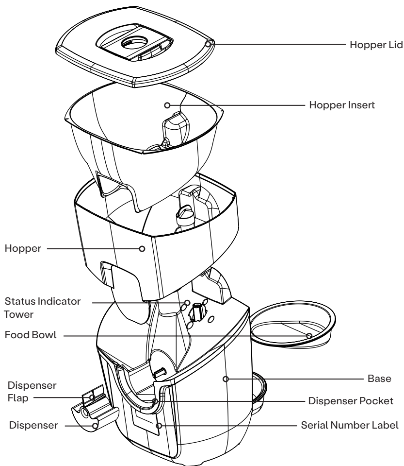
Exploded View
